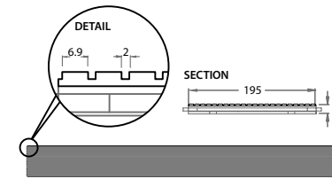
MULTI-RIGATO 2030x195 79,92"x7,68"
